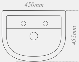
Monet Round semi-recessed cloakroom washbasin with integrated overflow and two tap holes, for use with a reduced depth fitted washbasin unit
